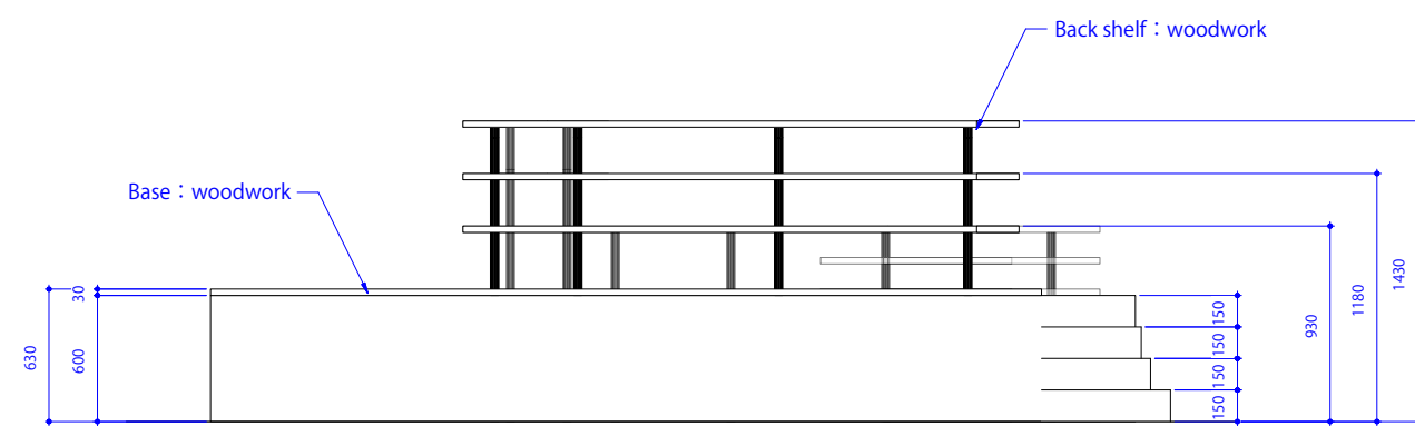
A-elevation
